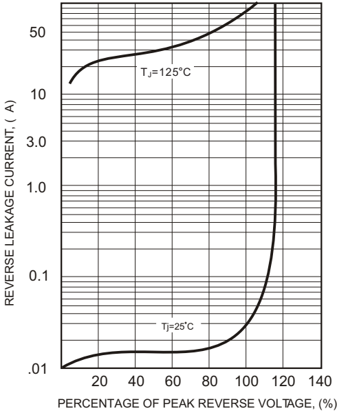
FIG.4-TYPICAL REVERSE CHARACTERISTICS
