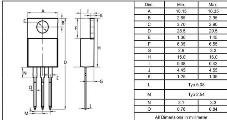
TO-220F
